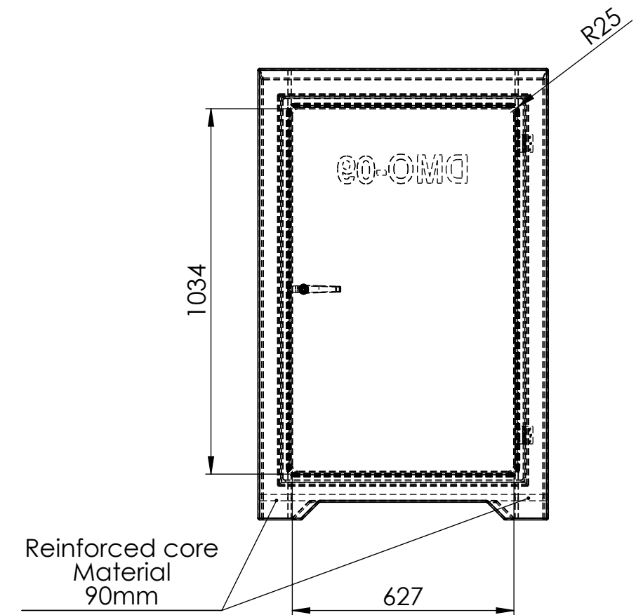
Rear View
